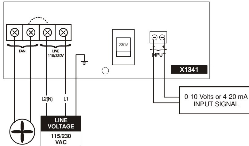
Figure 1: Wiring Diagram
