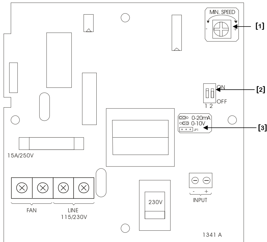
Figure 2: Electronic Board and Component Location
