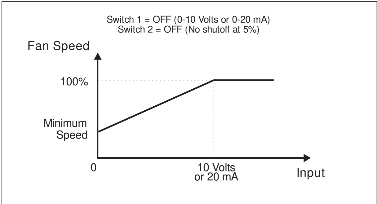
Figure 3: Logic Diagrams
